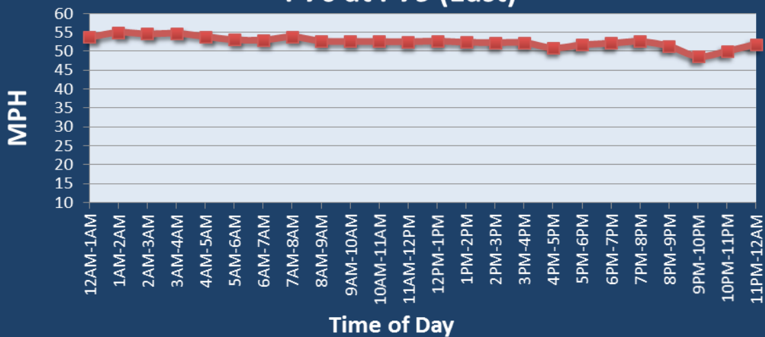
Average Speed by Time of Day I-70 at I-79 (East)
