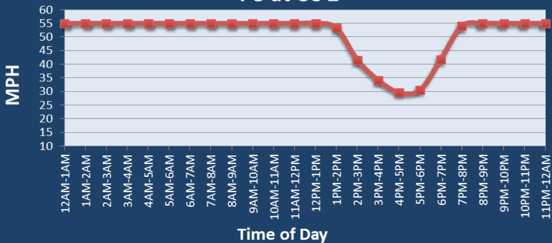
Average Speed by Time of Day I-5 at US 2
