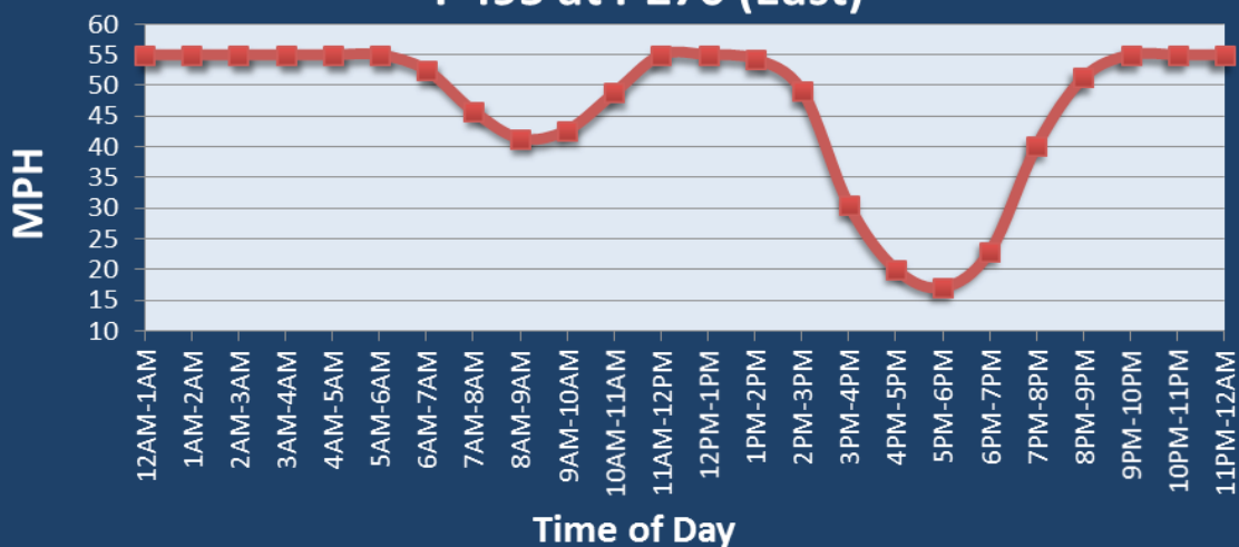
Average Speed by Time of Day I-495 at I-270 (East)
