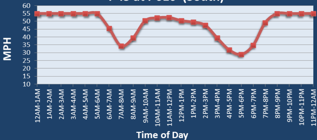
Average Speed by Time of Day I-45 at I-610 (South)
