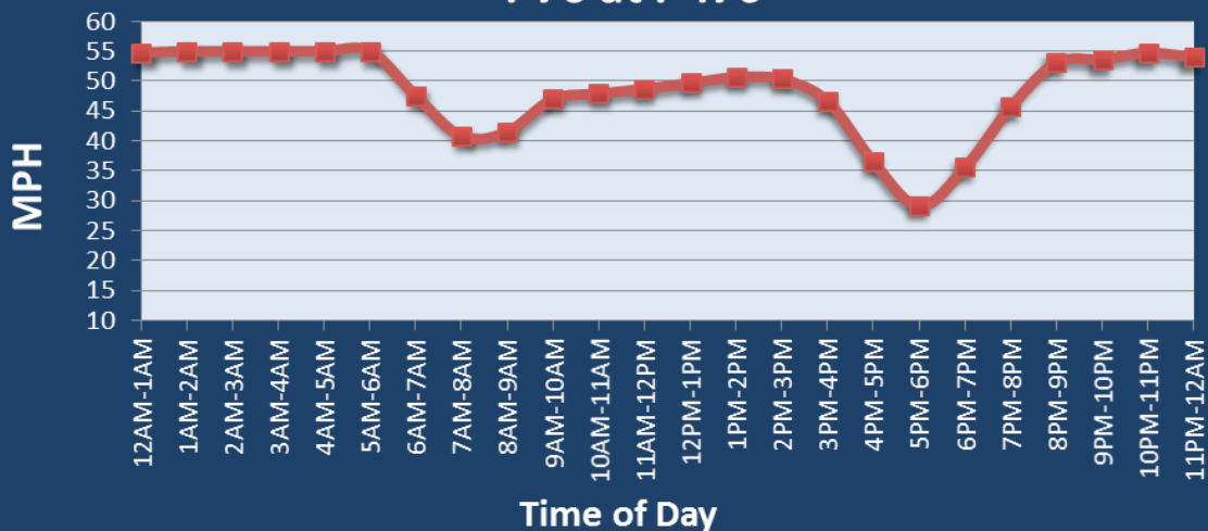
Average Speed by Time of Day I-76 at I-476
