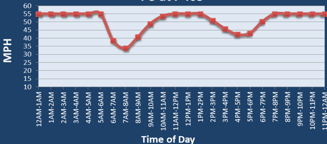
Average Speed by Time of Day I-5 at I-405
