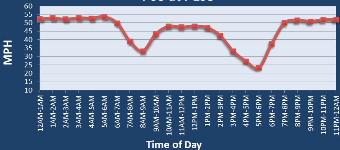
Average Speed by Time of Day I-95 at I-195
