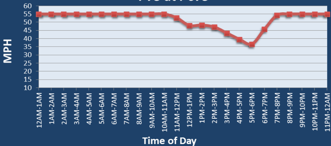
Average Speed by Time of Day I-75 at I-675
