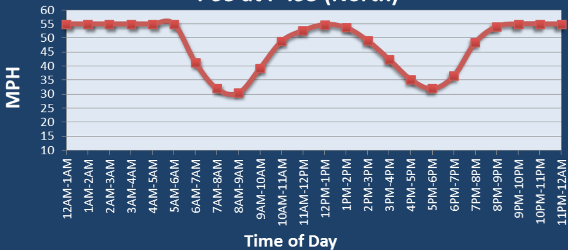
Average Speed by Time of Day I-95 at I-495 (North)
