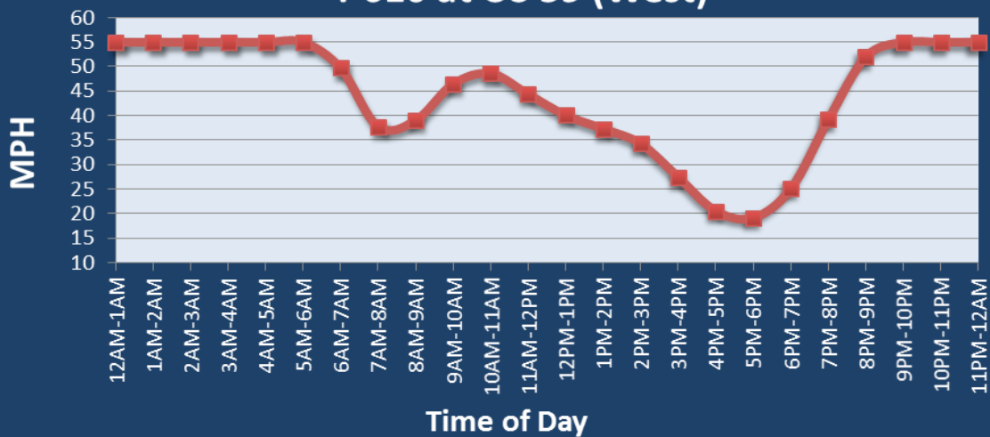
Average Speed by Time of Day I-610 at US 59 (West)
