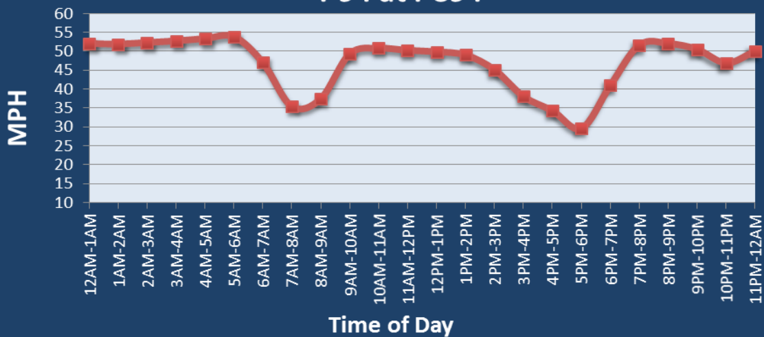
Average Speed by Time of Day I-94 at I-894
