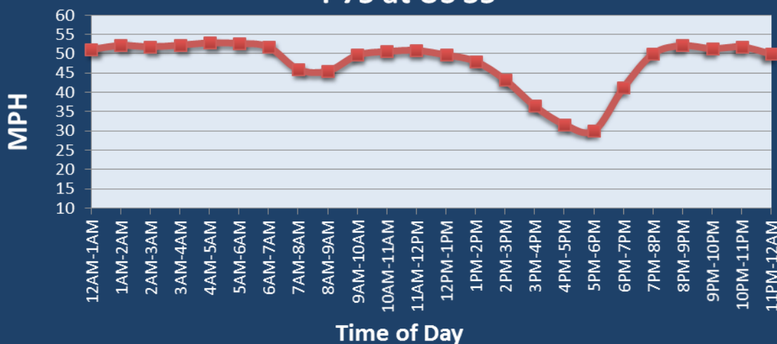
Average Speed by Time of Day I-75 at US 35
