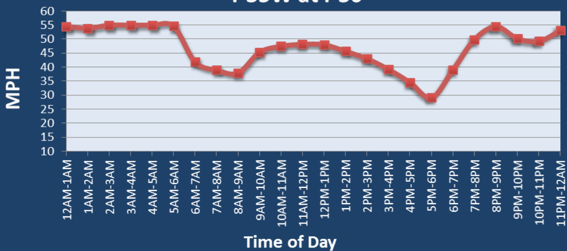
Average Speed by Time of Day I-35W at I-30
