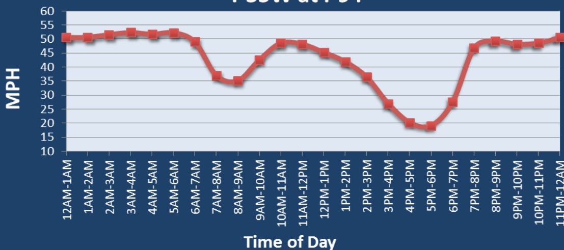
Average Speed by Time of Day I-35W at I-94
