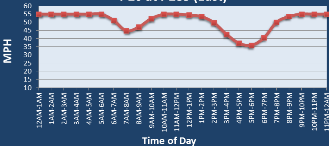
Average Speed by Time of Day I-20 at I-285 (East)
