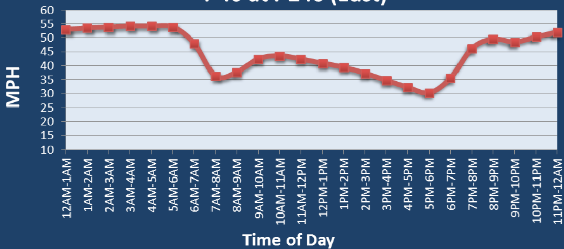
Average Speed by Time of Day I-40 at I-240 (East)
