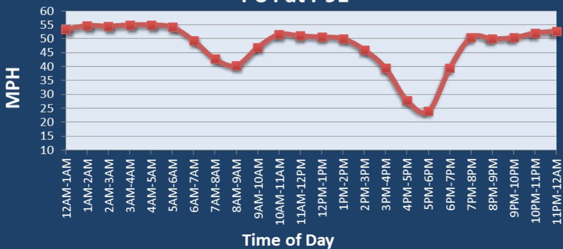
Average Speed by Time of Day I-84 at I-91
