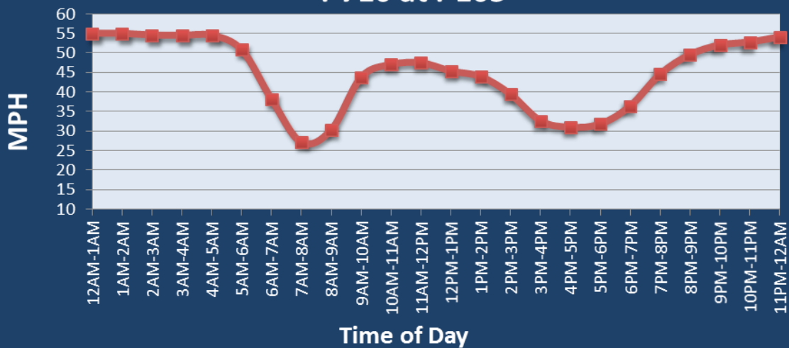
Average Speed by Time of Day I-710 at I-105
