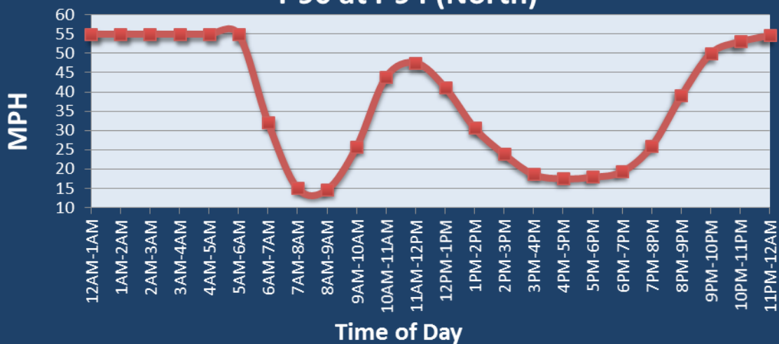
Average Speed by Time of Day I-90 at I-94 (North)
