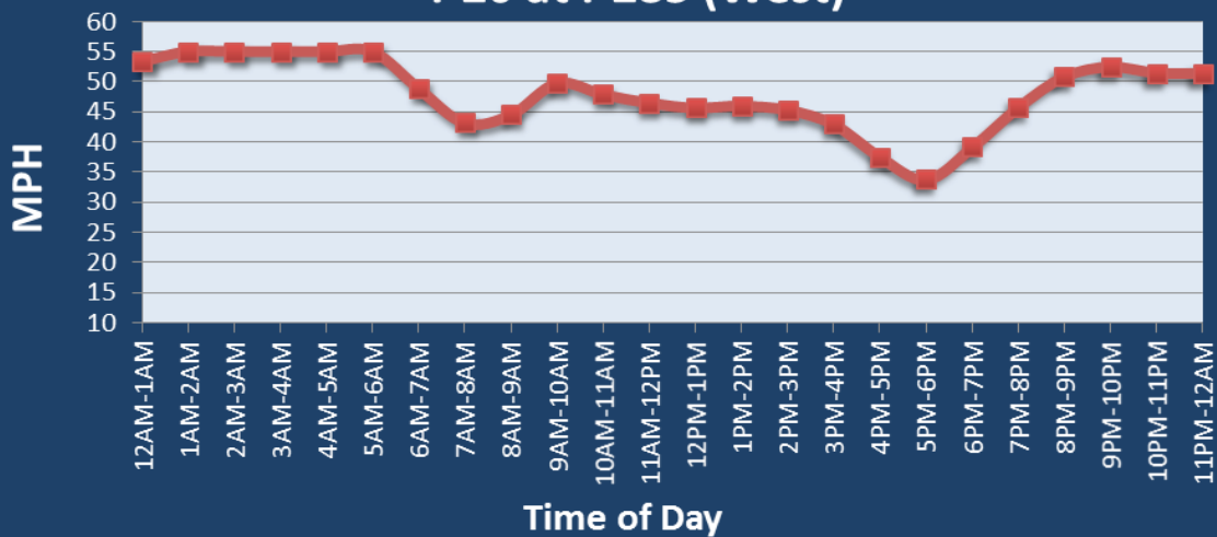
Average Speed by Time of Day I-20 at I-285 (West)
