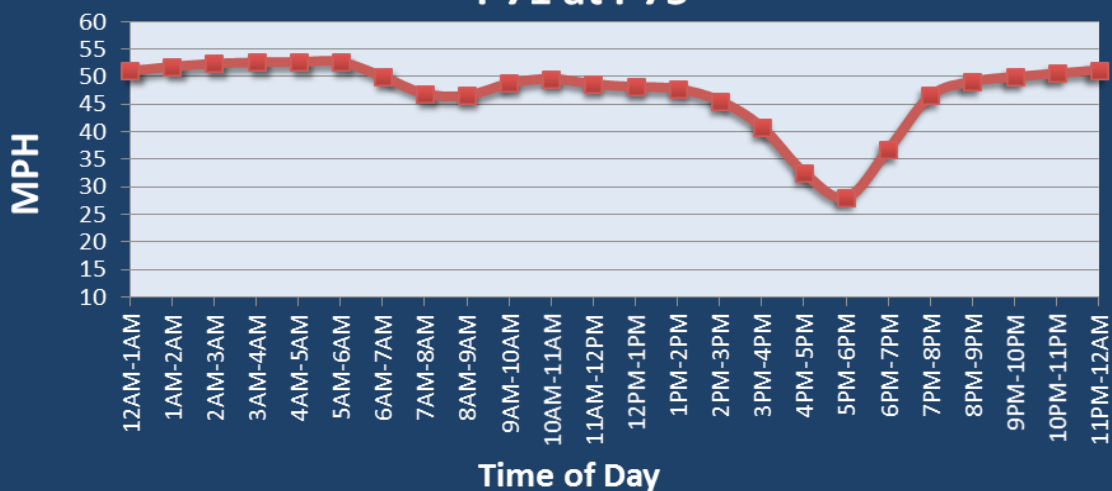
Average Speed by Time of Day I-71 at I-75
