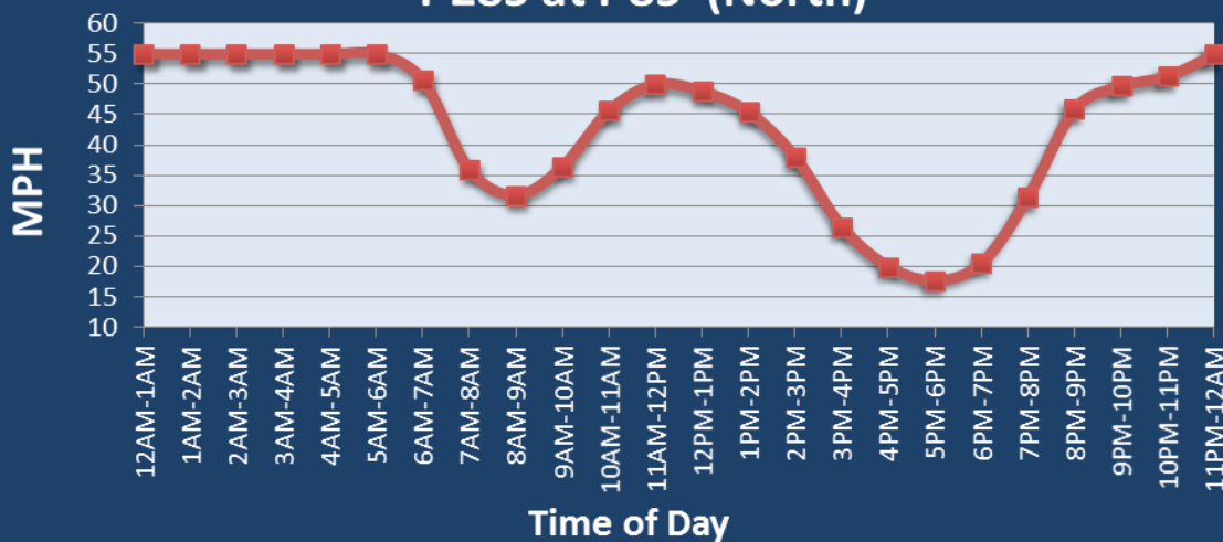
Average Speed by Time of Day I-285 at I-85 (North)
