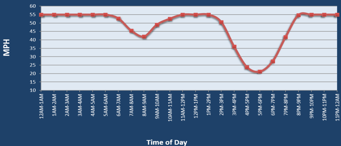
Average Speed by Time of Day I-495 at I-270 (East)
