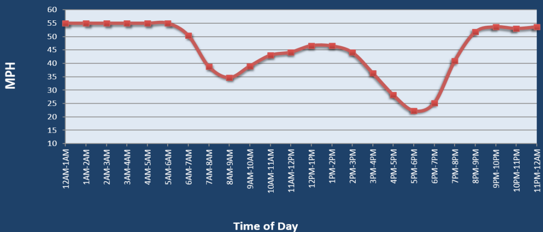
Average Speed by Time of Day I-495 at Shelter Rock Road
