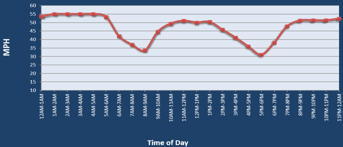
Average Speed by Time of Day I-95 at I-93 (North)
