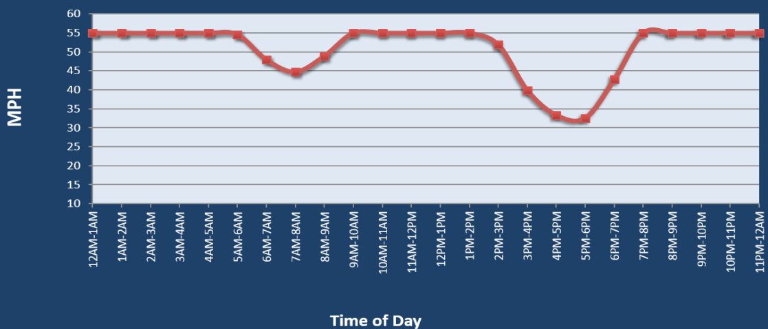
Average Speed by Time of Day I-17 at I-10
