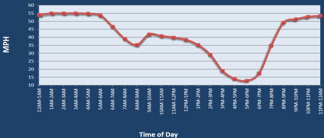
Average Speed by Time of Day I-80 at I-580/I-880
