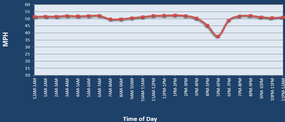
Average Speed by Time of Day I-65 at I-70 (South)
