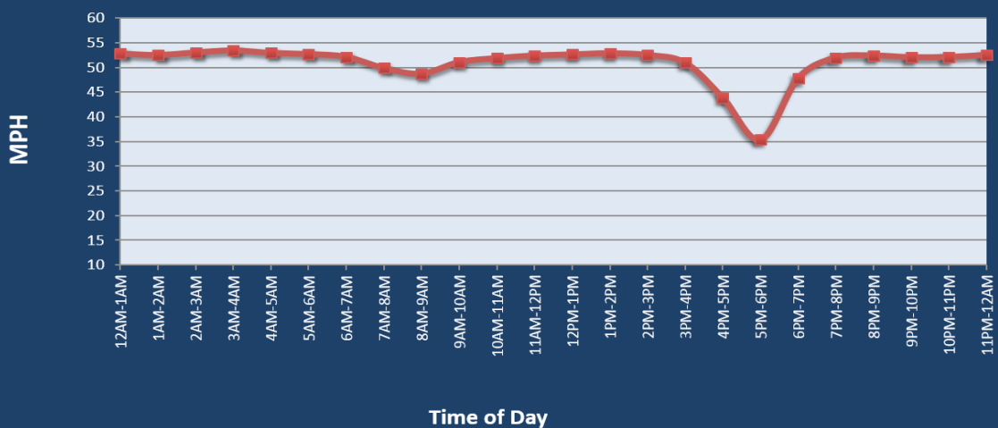
Average Speed by Time of Day I-65 at I-70 (North)
