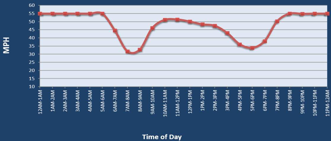
Average Speed by Time of Day I-45 at I-610 (North)
