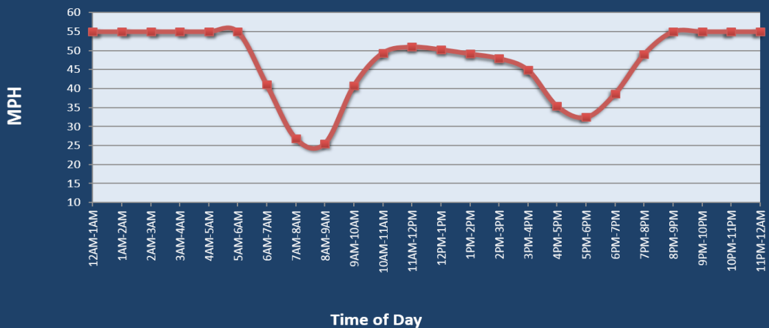
Average Speed by Time of Day I-10 at US 59
