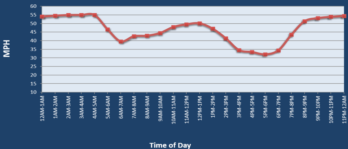
Average Speed by Time of Day SR 60 at SR 57
